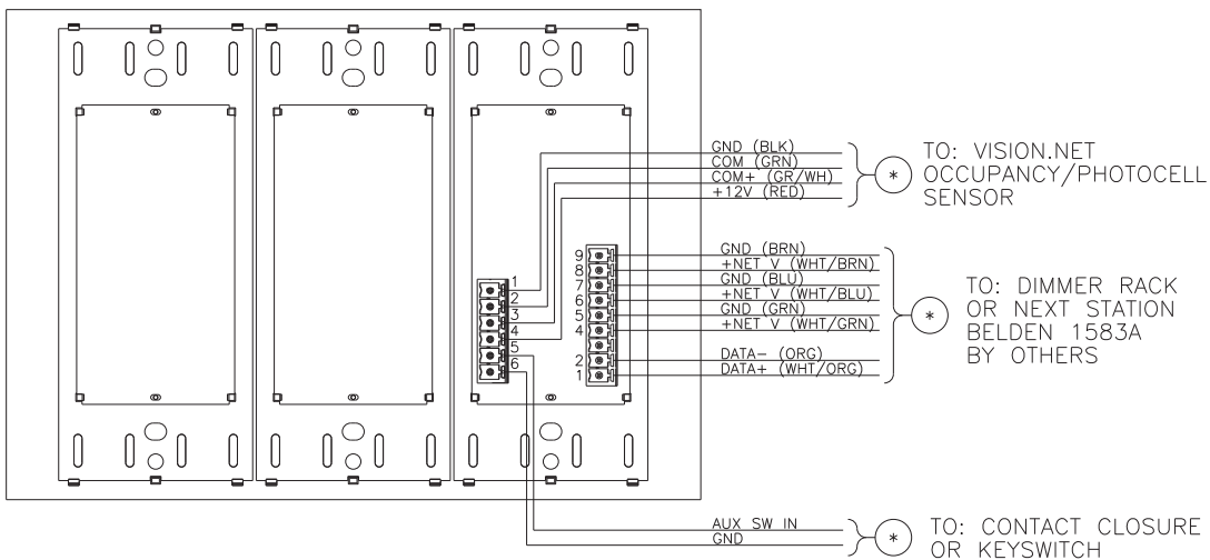
EXAMPLE 3-GANG WIRING
