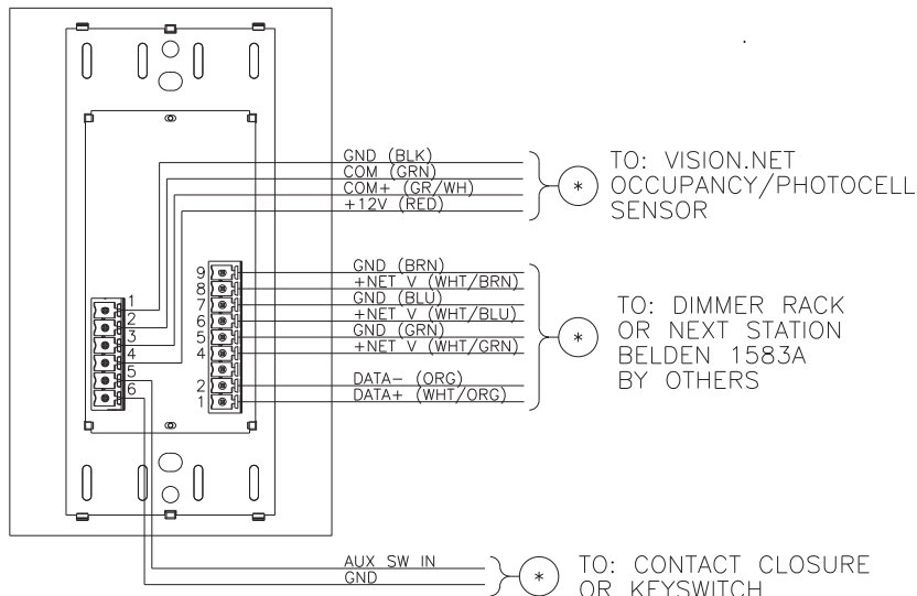
EXAMPLE 1-GANG WIRING
